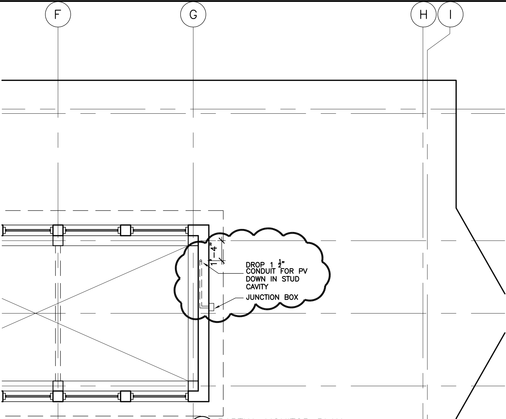
1 PARTIAL MONITOR PLAN 1/4" = 1'-0"
