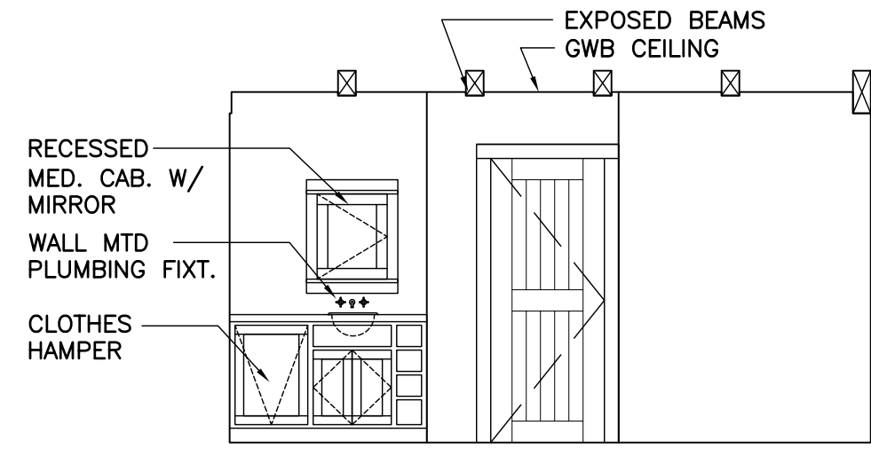
03 INT. ELEVATION @ BATH 09 SCALE: 1/4" = 1'-0"
